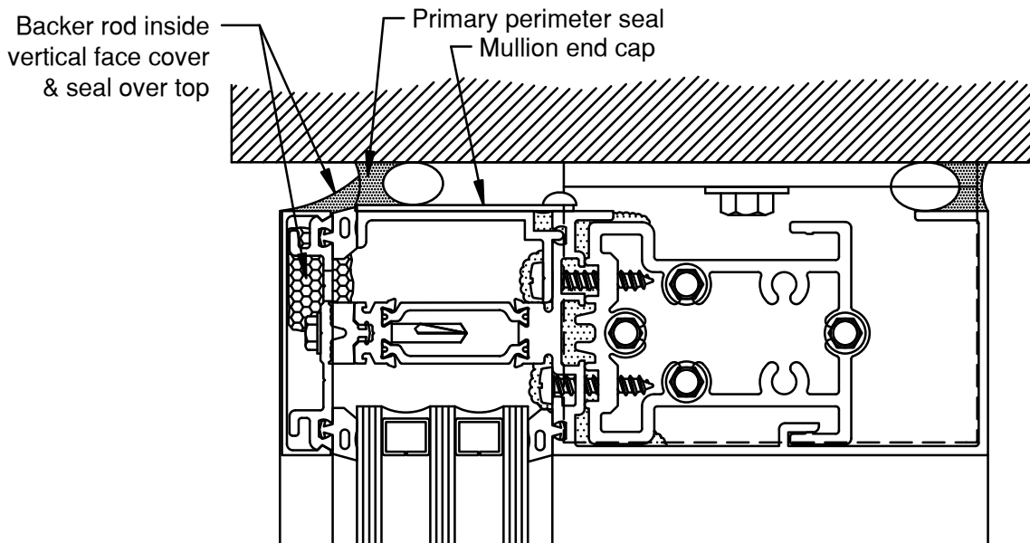
FIGURE 17 Sealing Top of Captured Verticals
