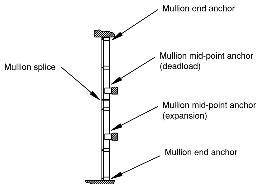
Multi-Span Refer to steps 2.1.6 through 2.1.13
