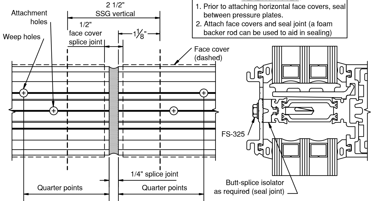
Pressure Plate Splice
