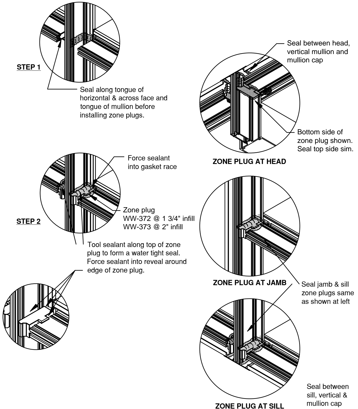
FIGURE 9 Zone Plug Installation
