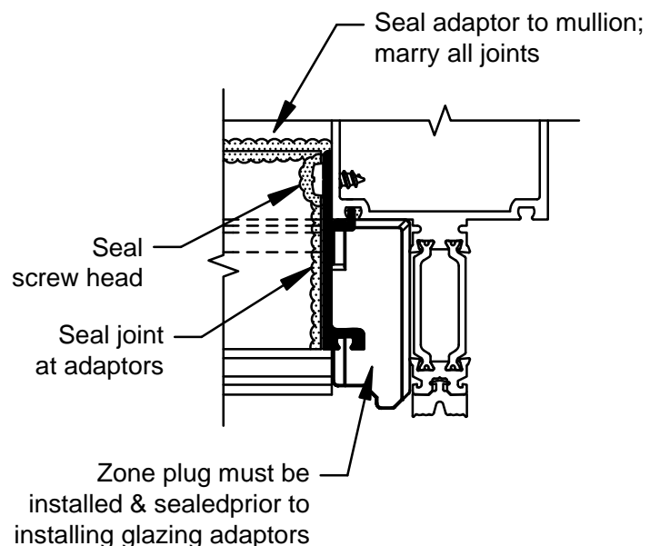
FIGURE 21 Sealing Glazing Adaptors
